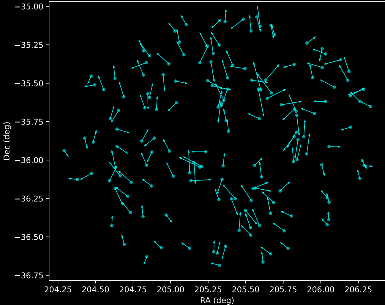
GALAH DR4 Noise Stream Proper Motion Vectors (n=152)
