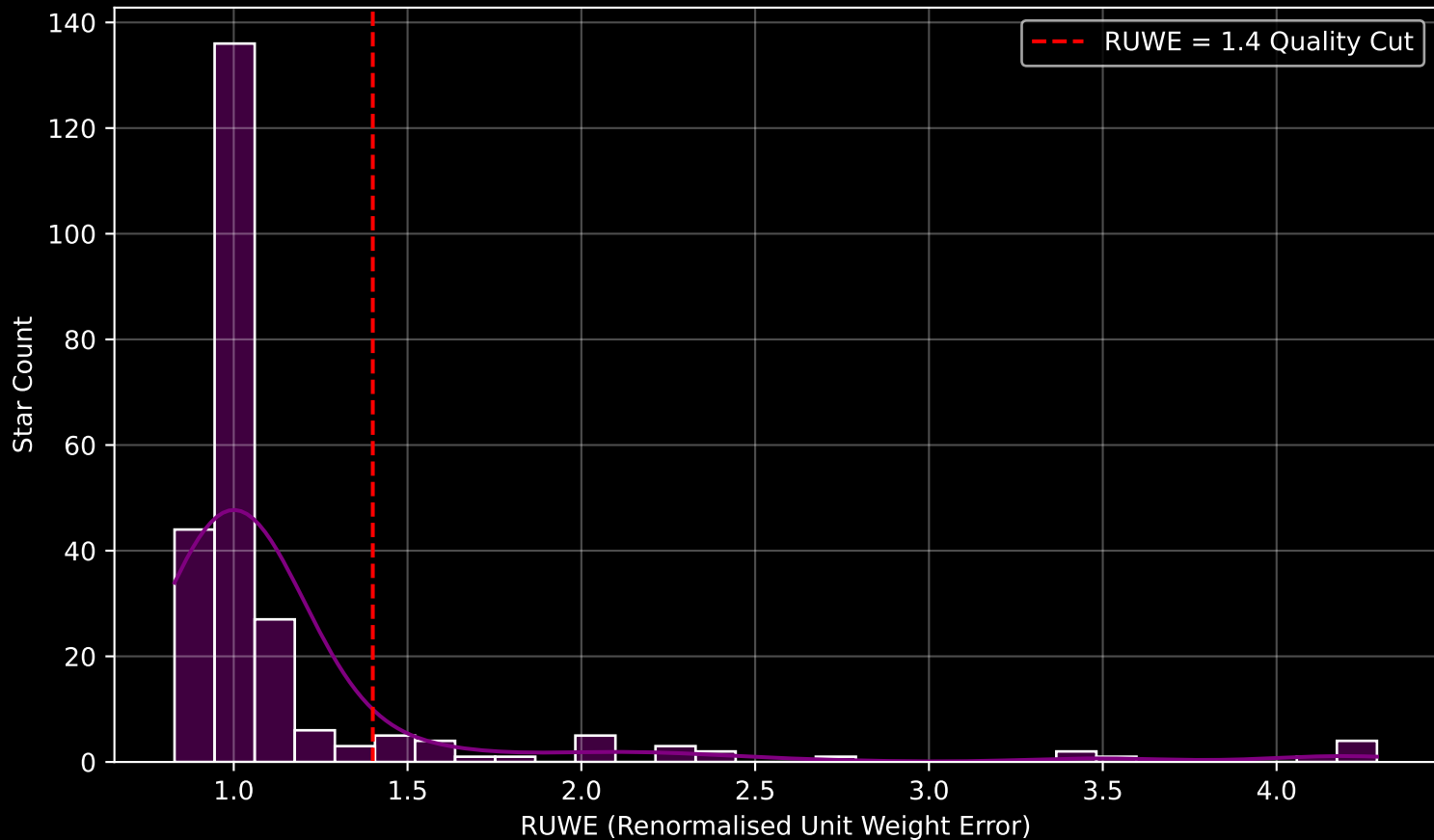
GALAH DR4 Field [3405] RUWE Distribution (n= 246)
