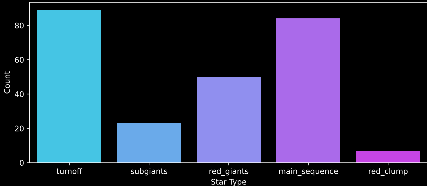
GALAH DR4 Field: [3405] Count plot of Star Type
