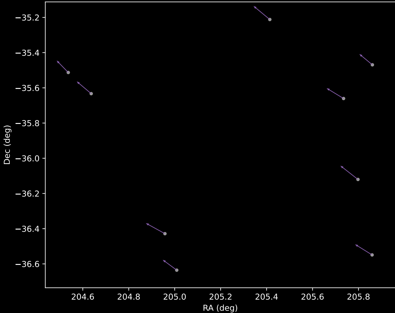
GALAH DR4 Cluster 8 Proper Motion Vectors (n=9)
